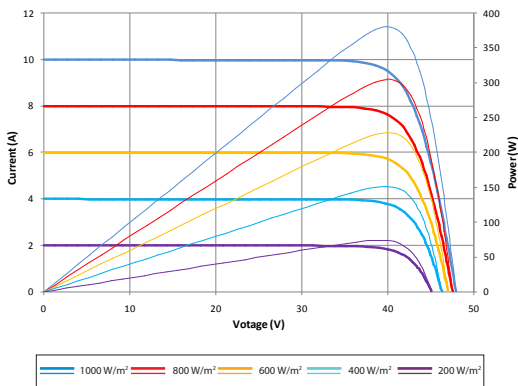
Current-Voltage & Power-Voltage Curve (380S)
